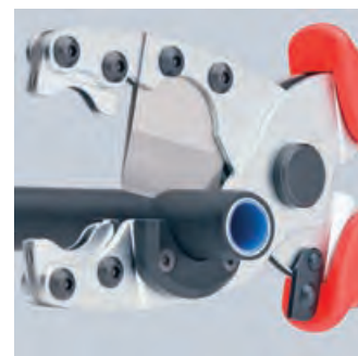
Composite pipes of 12 - 25 mm dia. are cut cleanly and without deformation
